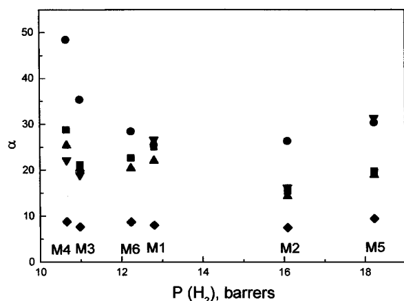
Figure 9. Variation of the (●) \alpha(H_2/N_2) , (■) \alpha(H_2/CO) , (▲) \alpha(H_2/CH_4) , (▼) \alpha(H_2/C_2H_4) , and (◆) \alpha(H_2/O_2) with the permeability of hydrogen in different membranes.
